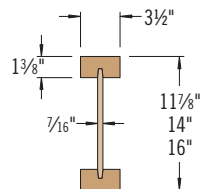
TJI® 560 joists
