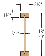
TJI® 560 Joist
