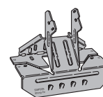
Variable Slope Seat Connector
