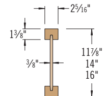
TJI® 360 joists
