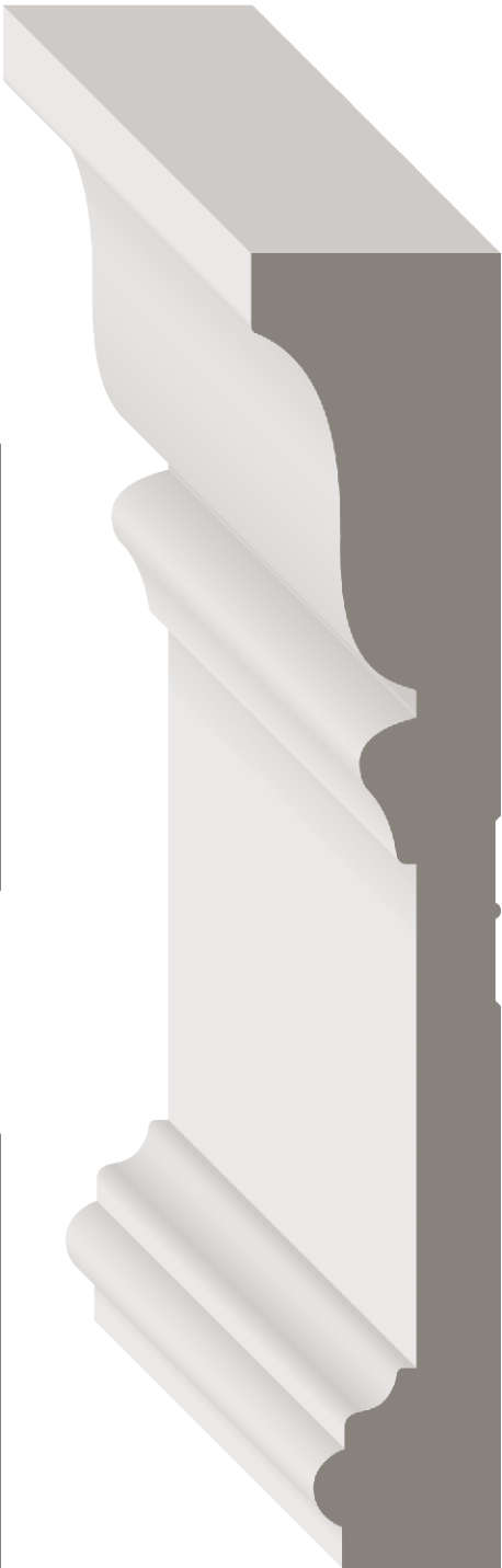
Stock Code Dimensions 5030M 1⅞" x 6¼" x 16' (1382895) MDF/UL
