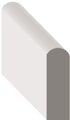
Stock Code 954LPOP (1485115) Dimensions \frac{7}{16} " x 1\frac{3}{8} " x RL POP
